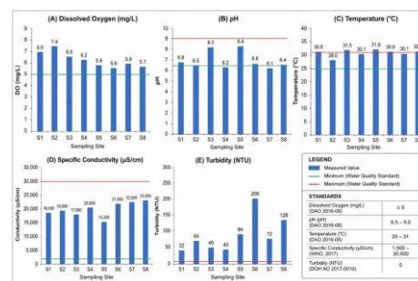
Figure 2. Graph in dissolved oxygen, pH, temperature specific conductivity, and turbidity among sampling sites in Lake Buluan.
